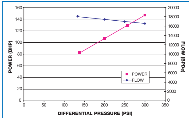
Flow and Power vs Pressure L4MK 144 (@100 cSt, 1750 RPM)
