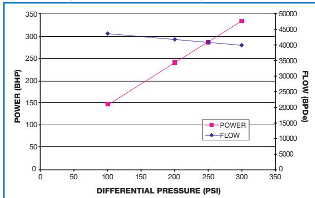
Flow and Power vs Pressure L4MK 186 (@100 cSt, 1750 RPM)
